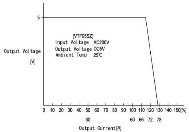
OCP Curve
