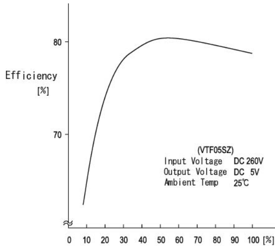
Efficiency Curve
