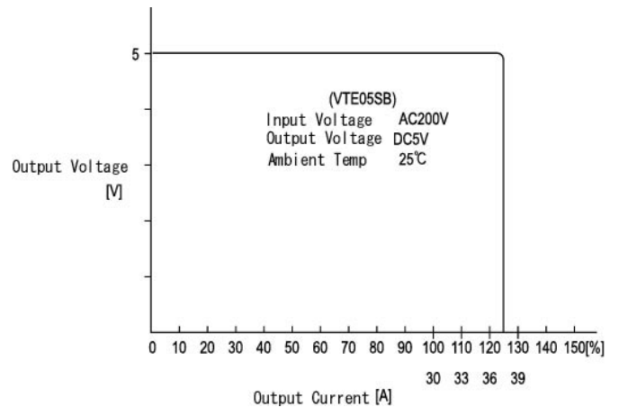
OCP Curve
